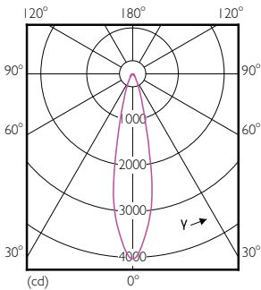
LED Classic PAR38 12W E26 835 F25
