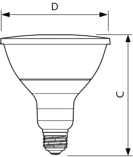
PAR38 120V 11-90W 900lm 25D 3500K E26 D
