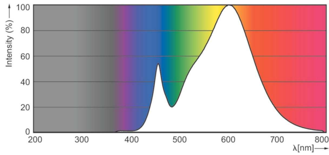
LEDlamps 6-50W PAR20 E26 3000K 500lm
