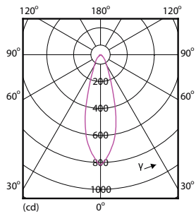
LEDspot PAR20 7W 830 500lm 25D
