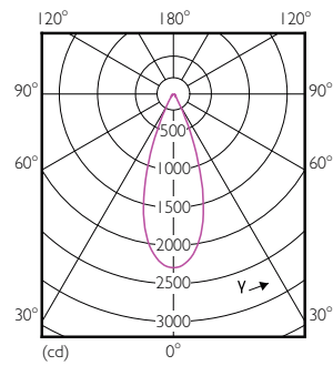
PAR30S 12W 950lm 40D 2700K E26
