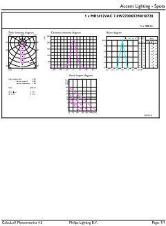
LEDspot 7.8W GU5.3 MR16 927 25D DIM
