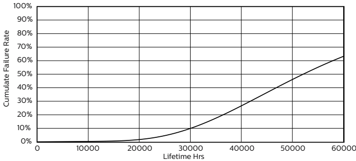
LEDtube 1200mm 14-32W G13
