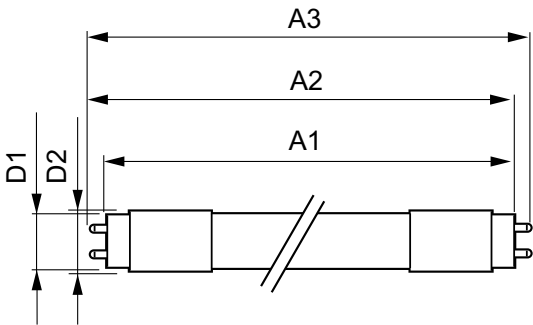
TLED 1200mm 120V 14-32W 2100lm 4000K G13
