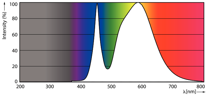
High Intensity 40W E39 ED-28 Clear 4000K
