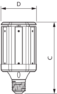
H L Bulb 40W-100W 5000lm 4000K E39 ND
