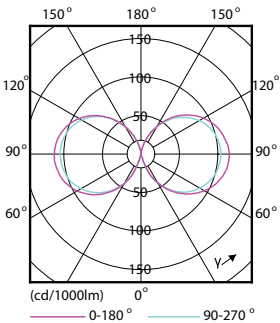
High Intensity 40W E39 ED-28 Clear 3000K
