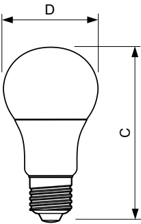
Bulb A19 120V 10W-75W 100D 2700K E26 ND
