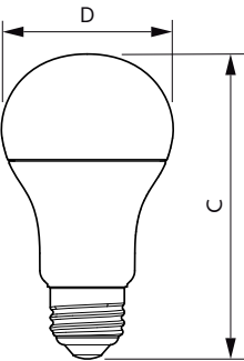
Bulb A60 11-75W 1000lm 2700K E26 ND
