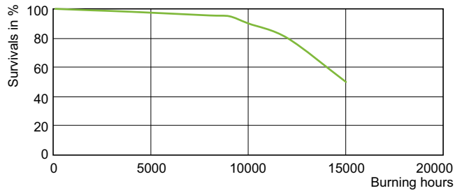
LDLE_CDM-R-E_930_PAR30L-Life expectancy diagram
