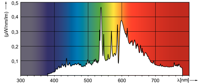
LDPO_CDM-T_150W_830-Spectral power distribution Colour
