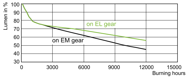
LDLM_CDM-T_150W_830-Lumen maintenance diagram
