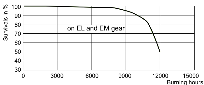
LDLE_CDM-T_150W_942-Life expectancy diagram
