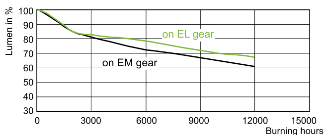
LDLM_CDM-T_150W_942-Lumen maintenance diagram
