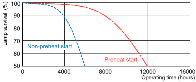
LDLE_TL5-C8_0001-Life expectancy diagram
