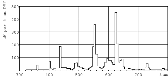
LDPB_TL5-C8_830-Spectral power distribution B/W
