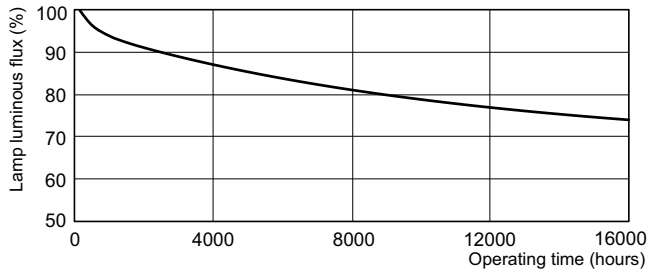
LDLM_TL5-C8_0001-Lumen maintenance diagram
