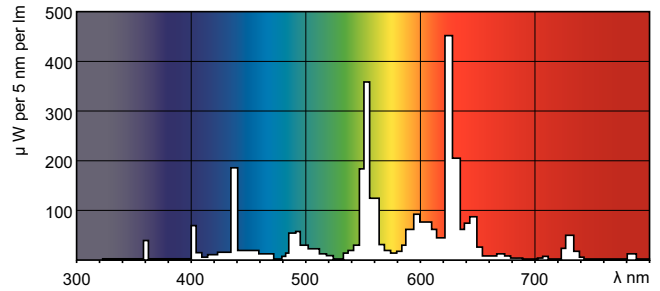
LDPO_TL5-C8_830-Spectral power distribution Colour
