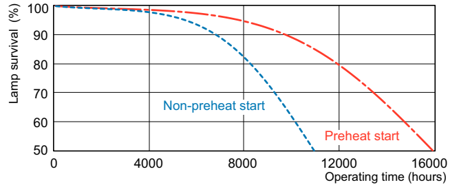
LDLE_TL5-C8_0002-Life expectancy diagram
