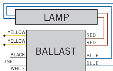
One Lamp Application, Cap Off Unused Leads Individually, Insulate to 600V
