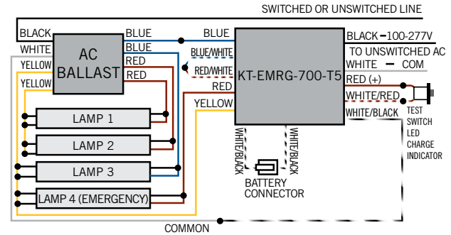
DIAGRAM 4-1 (Four Lamp Instant Start Ballast)
