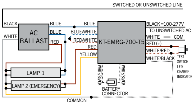
DIAGRAM 2-3 (Two Lamp Instant Start Ballast)
