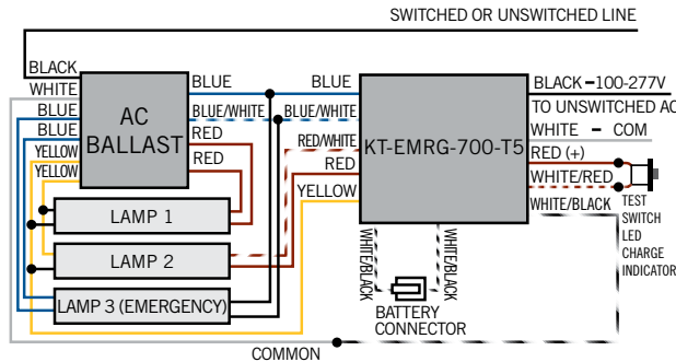
DIAGRAM 3-2 (Three Lamp Rapid Start Ballast)
